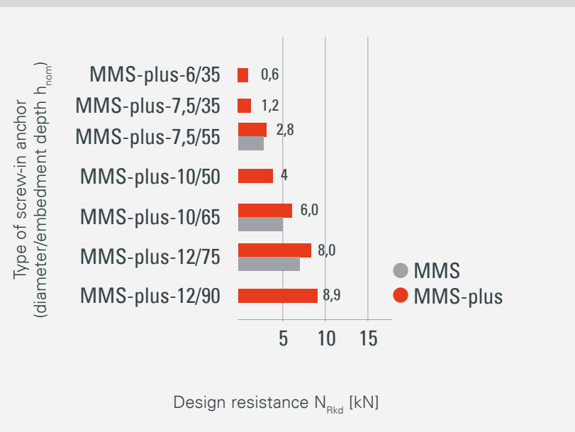
Pullout loads [kN] for cracked concrete C20/25
